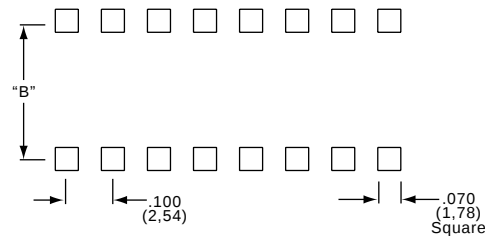
Recommended Pad Pattern Tolerance \pm .002 (0,05)
