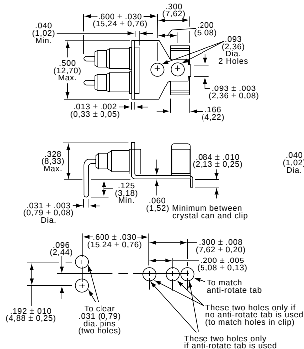
Cystal Outline Drawing
