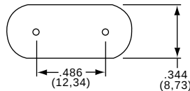
Crystal Outline Drawing
