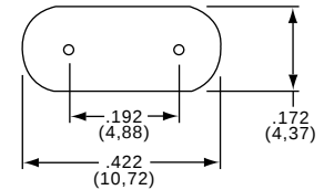
Crystal Outline Drawing
