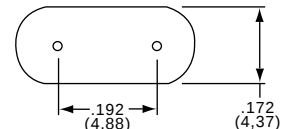
Cystal Outline Drawing
